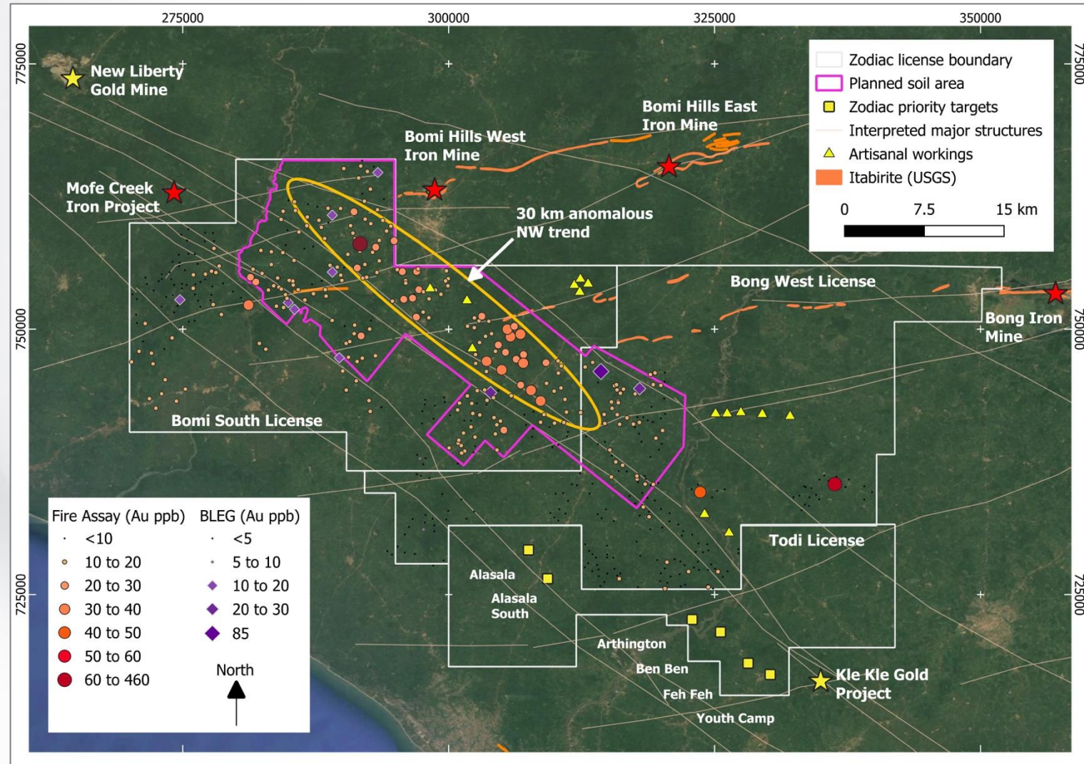
Zodiac license package with priority targets, stream sediment anomalism and current soil geochemical survey area
