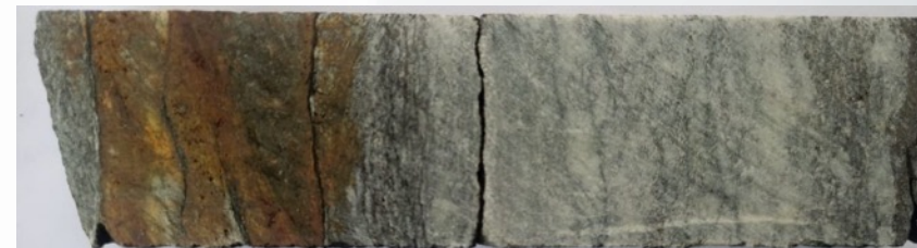
ADD024: 103.00 m-104.14 m sample interval with 16.80 g/t Au
